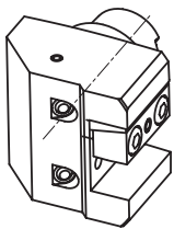
Axial toolholder 25x25 mm 142-11402
