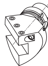
Toolholder 45° 25x25 mm 141-11407 (left) 141-21401 (right)
