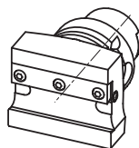
Radial toolholder for cut off tools 147-51409 (26mm) 147-51410 (32mm)
