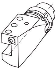
Axial toolholder 25x25 mm 142-21401 (left) 142-11403 (right)
