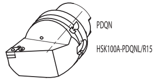
PDJN HSK100A-PDJNL/R15
