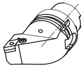
PDJN H63APDJNL/R15-OM
